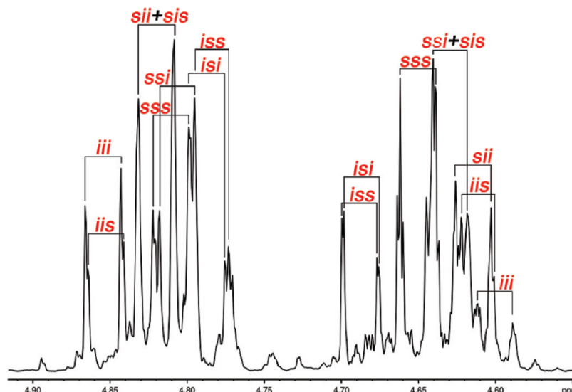
Figure 14. Glycolic methylene region of poly \text{L}_{\text{rac}}\text{L}_{\text{rac}}\text{G} at 700 MHz in \text{CDCl}_3 .
