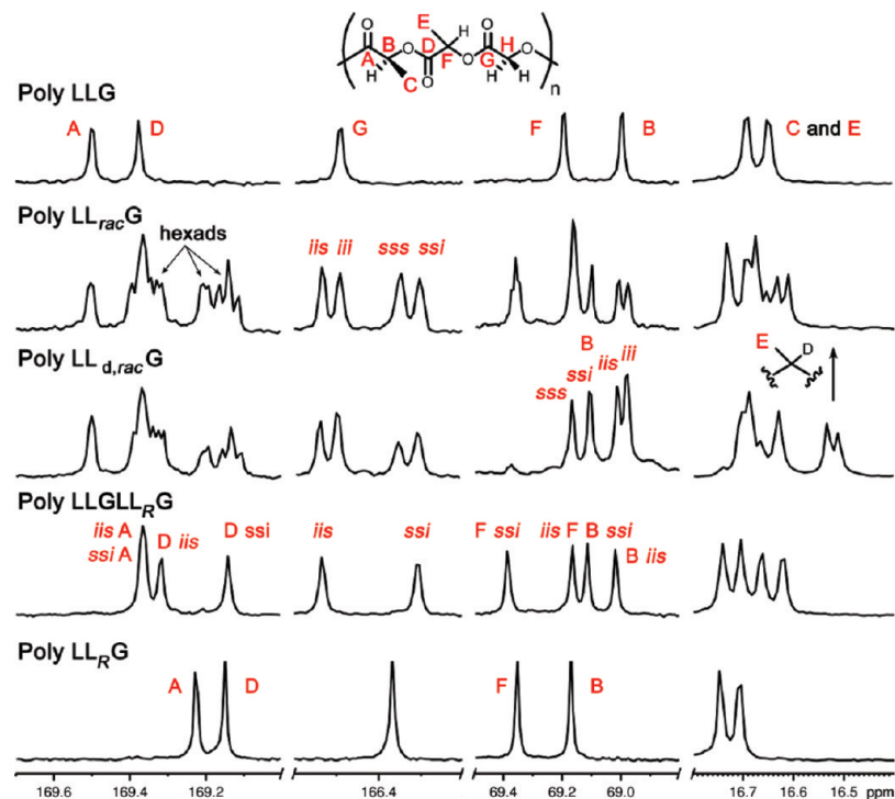
Figure 12. ^{13}\text{C} NMR spectra of \text{L}^{\text{C}} -variable LLG polymers at 175 MHz in \text{CDCl}_3 . Comparisons of the expansions of selected regions for poly LLG , \text{LL}_{\text{rac}}\text{G} , \text{LL}_{\text{d,rac}}\text{G} , \text{LL}_{\text{R}}\text{GLLG} , and \text{LL}_{\text{R}}\text{G} .
