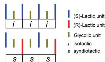
Figure 3. Example of tetrad stereosequence encoding for poly LG (all isotactic) and GLGL R (all syndiotactic).
