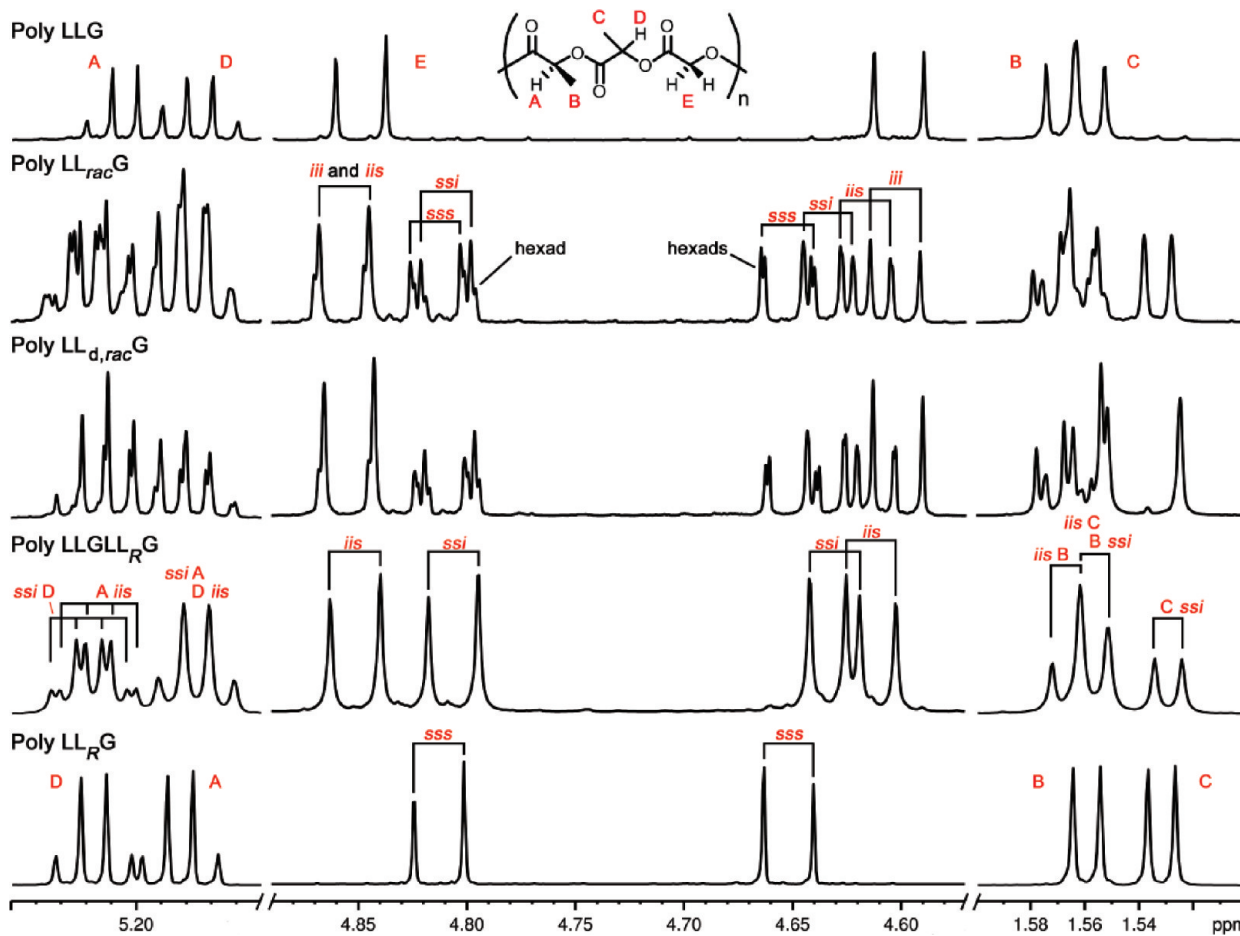
Figure 8. ^1\text{H} NMR spectra of \text{L}^{\text{C}} -variable LLG polymers at 700 MHz in \text{CDCl}_3 . Comparisons of the expansions of selected regions for poly LLG , \text{LL}_{\text{rac}}\text{G} , \text{LL}_{\text{d,rac}}\text{G} , \text{LLGLL}_R\text{G} , and \text{LL}_R\text{G} .
