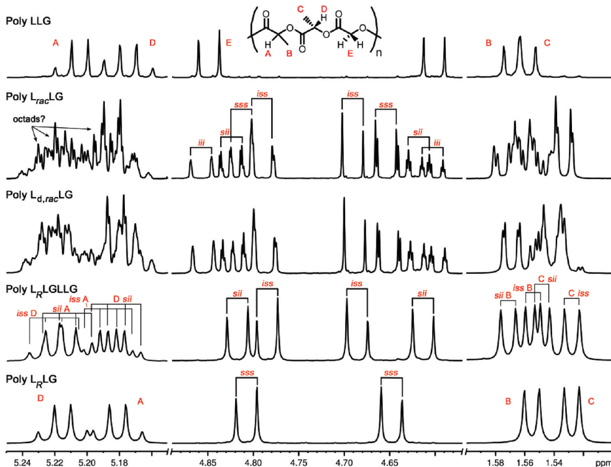
Figure 7. ^1\text{H} NMR spectra of \text{L}^{\text{O}} -variable LLG polymers at 700 MHz in \text{CDCl}_3 . Comparisons of the expansions of selected regions for poly LLG , \text{L}_{\text{rac}}\text{LG} , \text{L}_{\text{d,rac}}\text{LG} , \text{L}_{\text{R}}\text{LGLLG} , and \text{L}_{\text{R}}\text{LG} .
