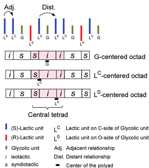
Figure 6. Example of octad-level stereosequence encoding for poly L R L S GL S L S G . The central tetrads for each type of unit are defined as including one distant and two adjacent relationships.
